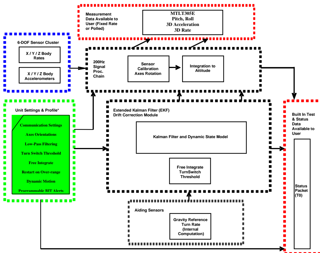
Figure 4 MTLT305E Series Software Block Diagram
