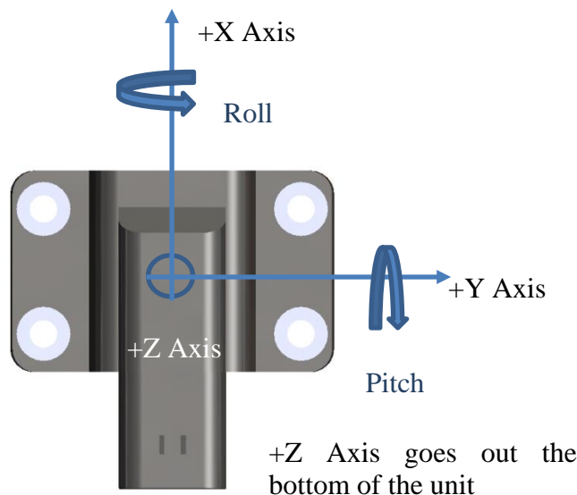
Figure 5. MTLT305E Default Coordinate Frame
