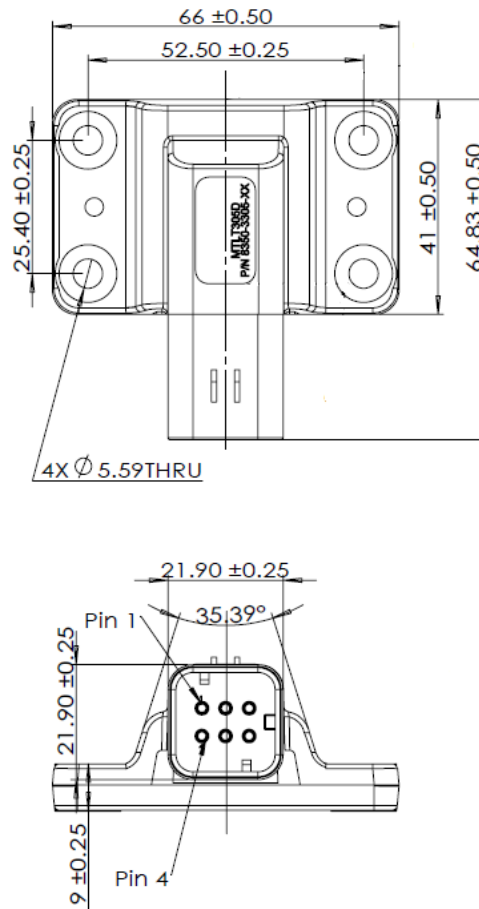
Figure 2 MTLT305E Outline Drawing
