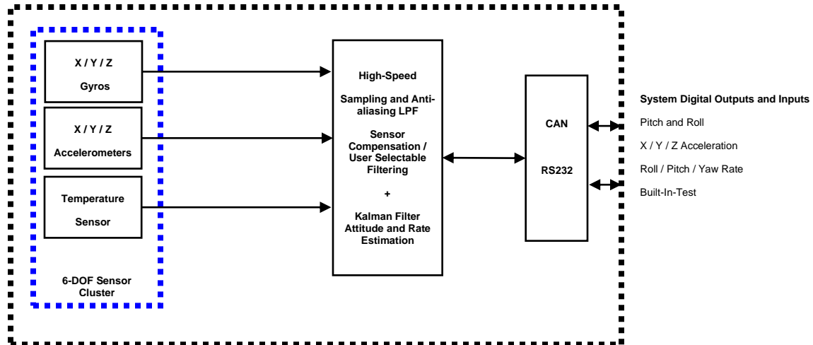
Figure 3 MTLT305E Series Hardware Block Diagram
