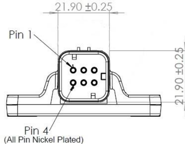
Figure 1 MTLT305E Interface Connector
