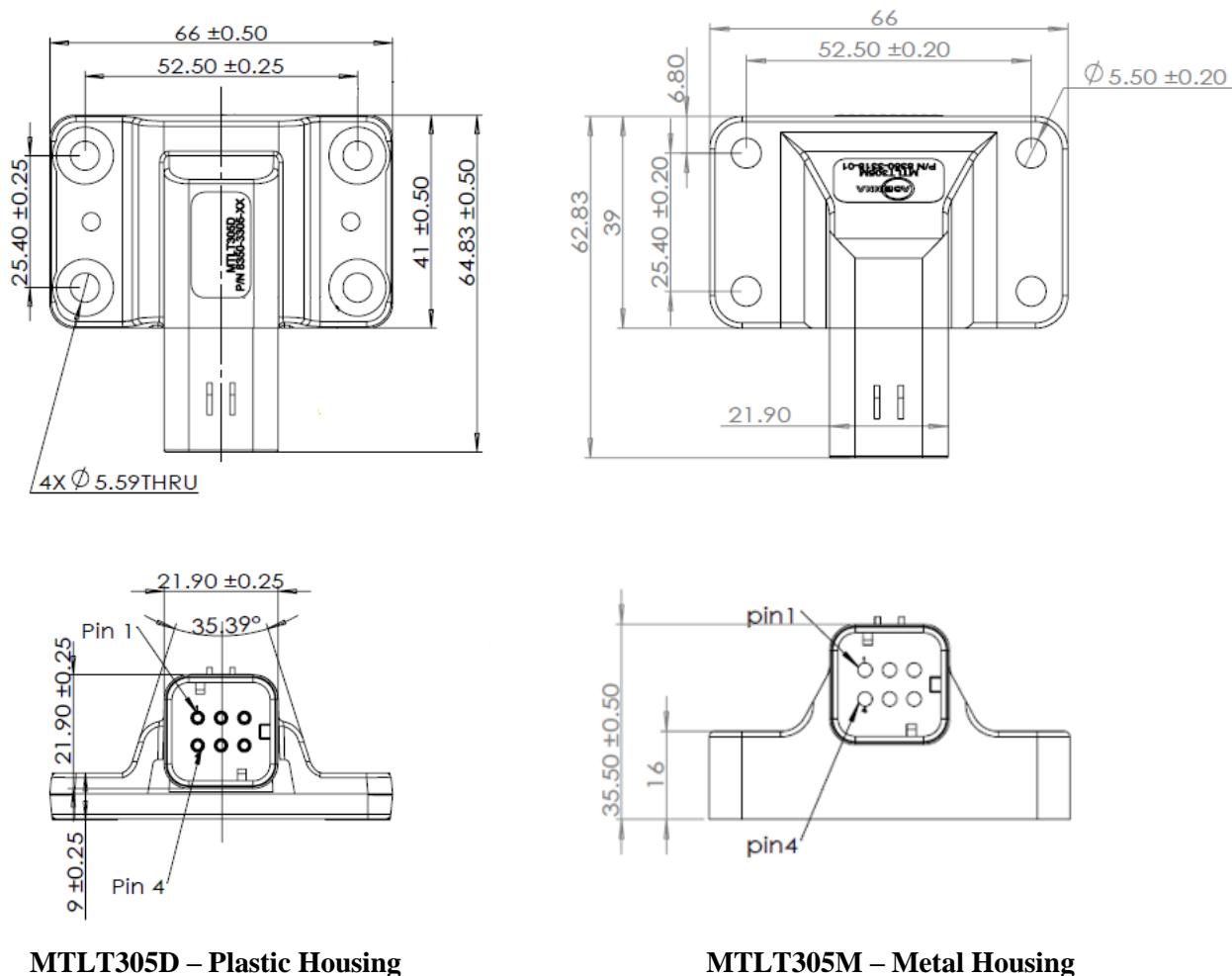
Figure 2 MTLT305D/M Outline Drawing
