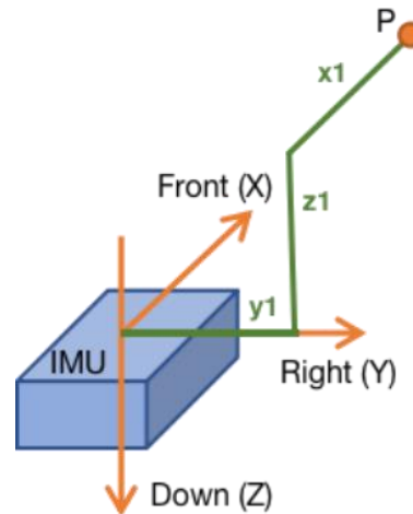
Figure 6. Case 1 Lever Arm Diagram
