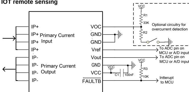
Figure 1 - Application Circuit
