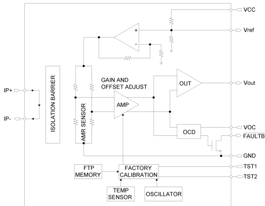
Figure 2 - Block diagram for fixed gain products
