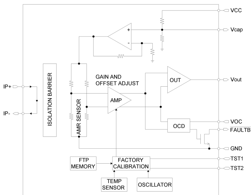
Figure 2 - Block diagram for ratiometric gain products
