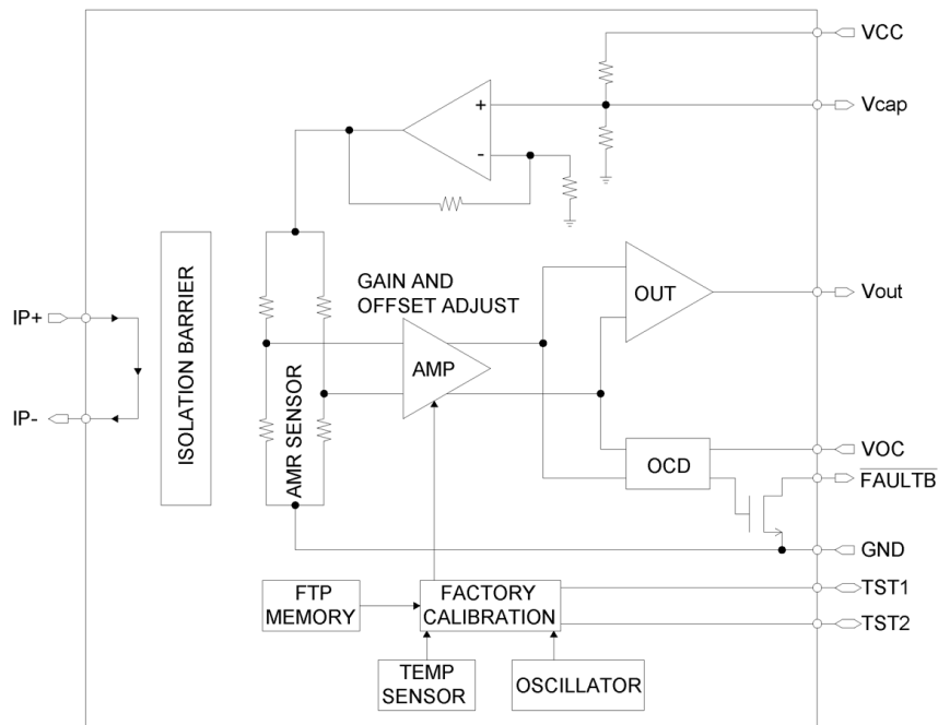
Figure 2 - Block diagram for ratiometric gain output products
