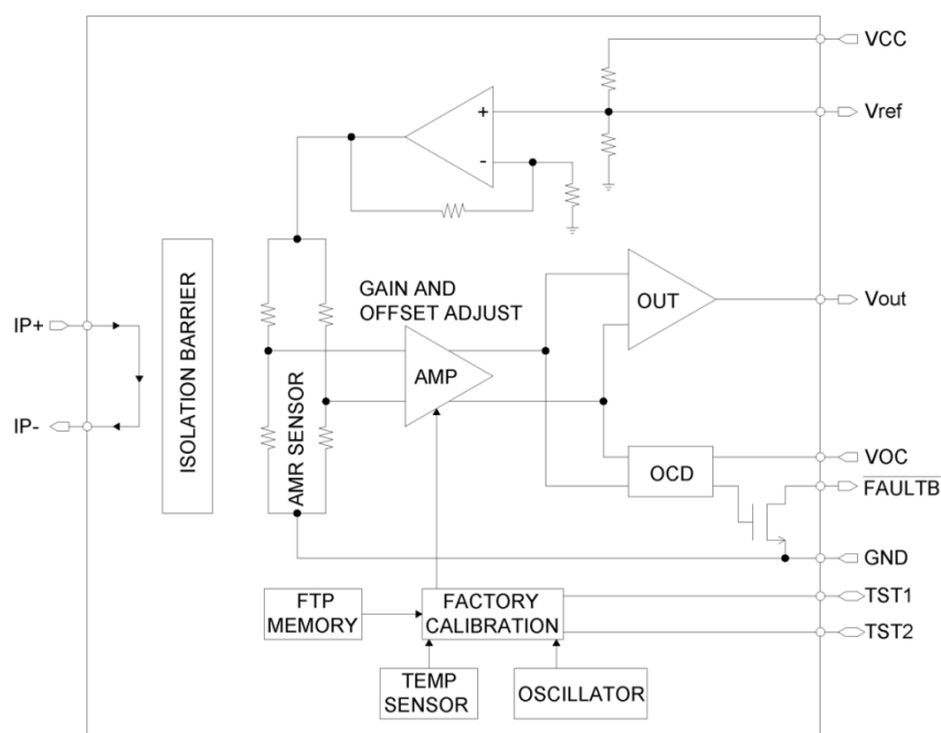
Figure 2 - Block diagram for fixed gain output products
