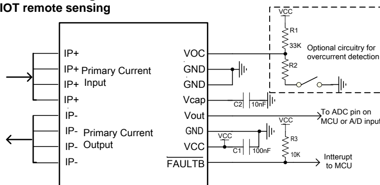
Figure 1 - Application Circuit
